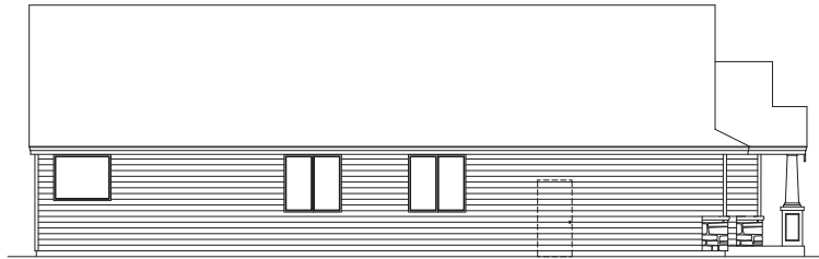
LEFT ELEVATION
